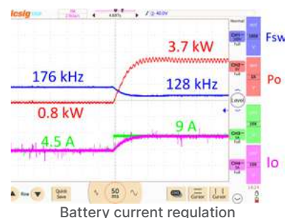
Battery current regulation
