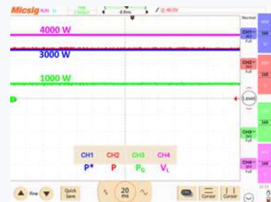
Power flow considering resistive load
