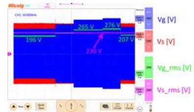
Voltage supply regulation with grid voltage variation
